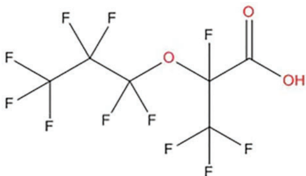
FIG. 1. Chemical structure of 2,3,3,3-tetrafluoro-2-(heptafluoropropoxy)-propanoate.
