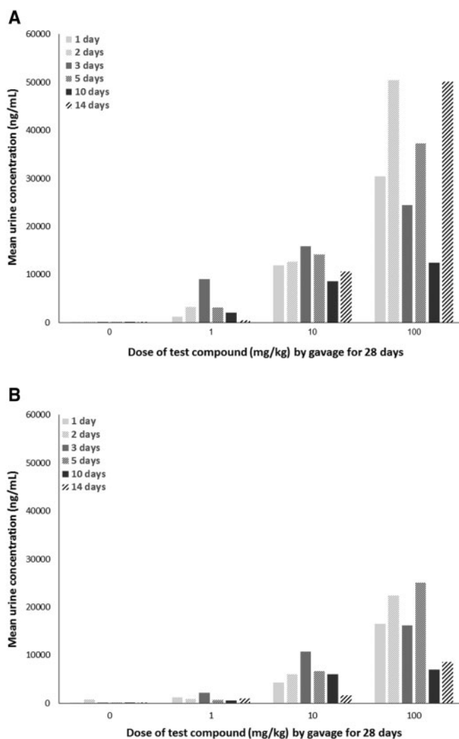
FIG. 7. Urine concentrations (mean) of male or female C57Bl/6 mice given 2,3,3,3-tetrafluoro-2-(heptafluoropropoxy)-propanoate via gavage for 28 days. Urine samples were collected after 1, 2, 3, 5, 10, and 14 days of exposure. A, Males. B, Females. Samples are pooled samples of 3 animals/sex/cage and 2 pooled samples/dose; sample sizes are, therefore, N = 1 or 2 /dose depending on the quantity of urine non-invasively excreted on a particular sample collection day.
